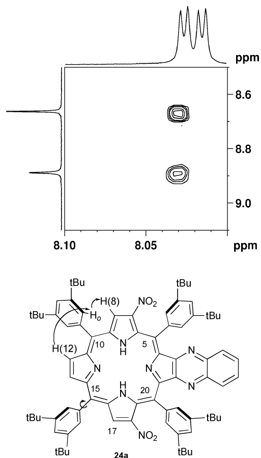
Fig. 1 Through-space connectivity of H(8)– H_o –H(12) seen in partial NOESY spectra of 7,18-dinitroporphyrin 24a .
