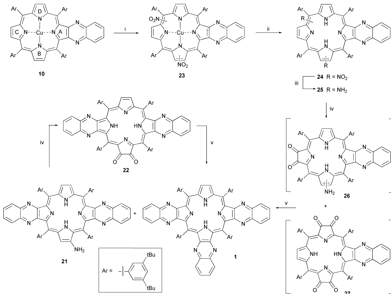
Scheme 4 Pathway 3, Reagents and conditions: (i) NO 2 in light petroleum, CH 2 H 2 ; (ii) H 2 SO 4 , CH 2 Cl 2 ; (iii) SnCl 2 ·2H 2 O in HCl–Et 2 O; (iv) O 2 , hν, CH 2 Cl 2 ; (v) 1,2-diaminobenzene, CH 2 Cl 2 .
